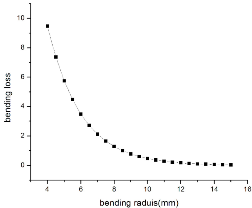
Figure: 3. bending radius vs. bending loss
