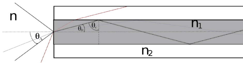
Figure: 1. A typical optical fiber waveguide consists of thin cylindrical glass rod [11]
