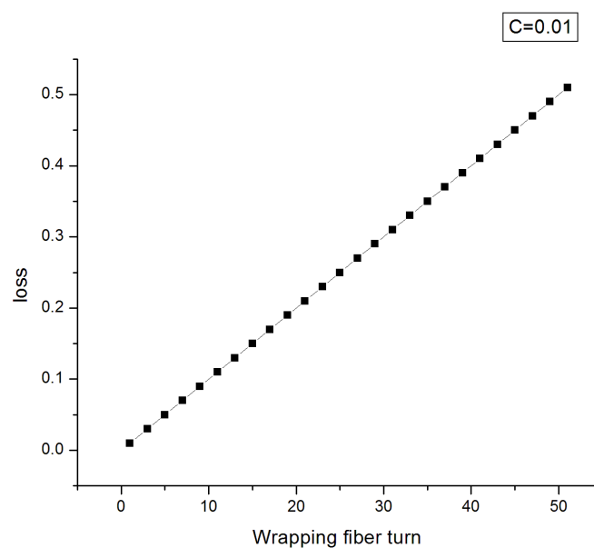
Figure: 4. Loss as a function of wrapping turns for step index single mode fiber
